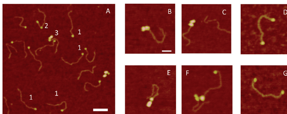
Figure 4. AFM images of complexes of SSB formed with the hybrid 69-tail-DNA under high-salt conditions. (A) Typical large-scale image on which different morphologies of complexes are indicated with 1–3. The bar is 100 nm. (B–G) Gallery of images of SSB–DNA complexes of various morphologies. The bar is 50 nm.
