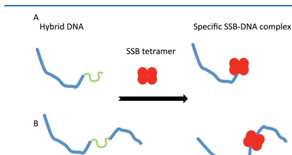
Figure 1. Schematic presentation of the formation of the complex between the SSB tetramer and (A) the tail-DNA substrate and (B) the gap-DNA substrate. DNA duplexes are shown as blue lines; ssDNA is depicted as green lines, and SSB is shown as red spheres.
