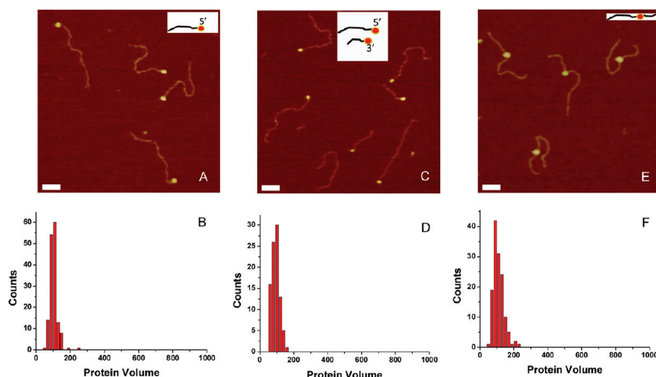
Figure 2. AFM data for complexes of SSB with hybrid DNA of different types. (A, C, and E) AFM images of complexes with 5'-tail-DNA, a mixture of 5'-tail-DNA and 3'-tail-DNA, and gap-DNA, respectively. The insets show the schematic presentations of all complexes. Bars are 50 nm. (B, D, and F) Histograms for the protein volumes for 5'-tail-DNA, a mixture of 5'-tail-DNA and 3'-tail-DNA, and gap-DNA, respectively.
