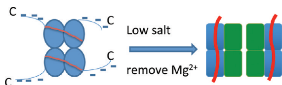
Figure 10. Schematic illustration of the salt-dependent conformational transition of SSB. Proteins are shown by ellipses of different shapes to illustrate the difference in the protein conformations under both conditions. At the left is the specific SSB–ssDNA complex. The protein C-termini are shown with blue lines. DNA is shown with red lines. At the right is the low-salt SSB–ssDNA complex. One dimer is shown in complex with DNA (red line). DNA is shown with red lines.
